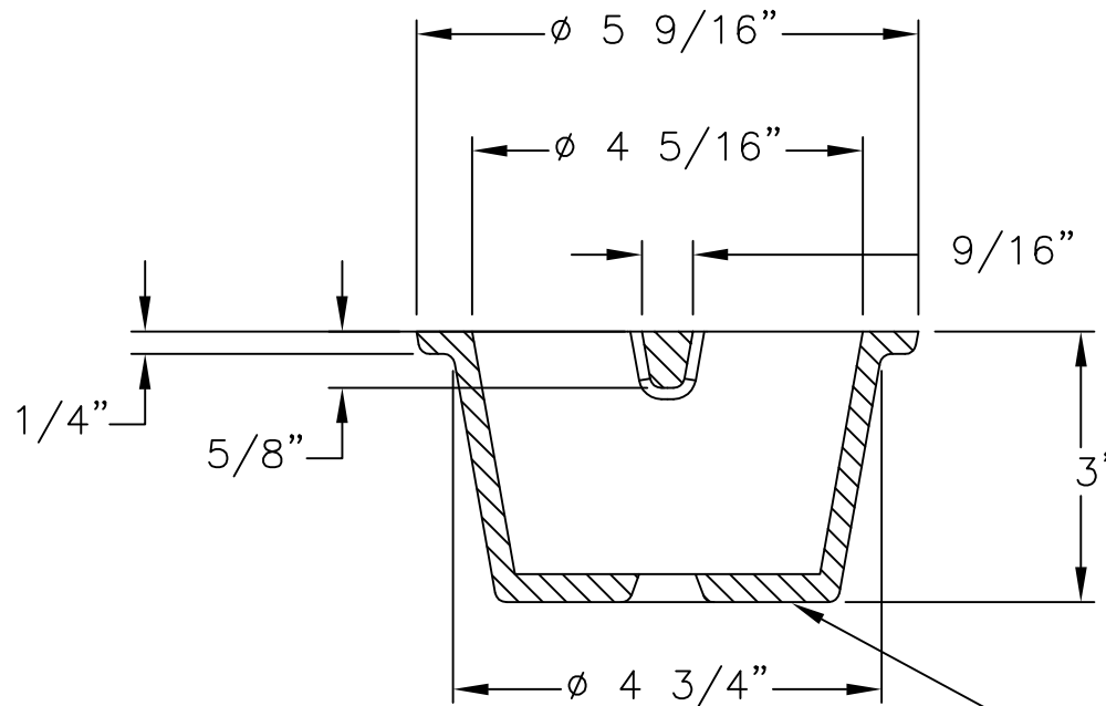
SECTION VIEW
