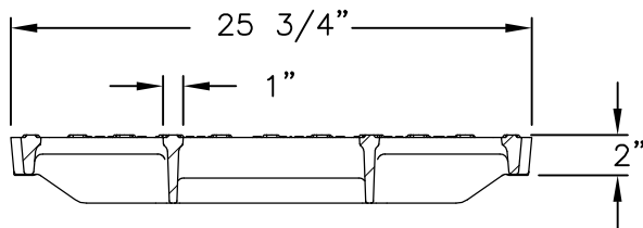
GRATE SECTION
