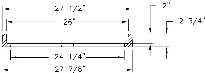
FRAME SECTION
