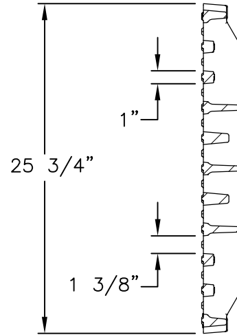
GRATE SECTION
