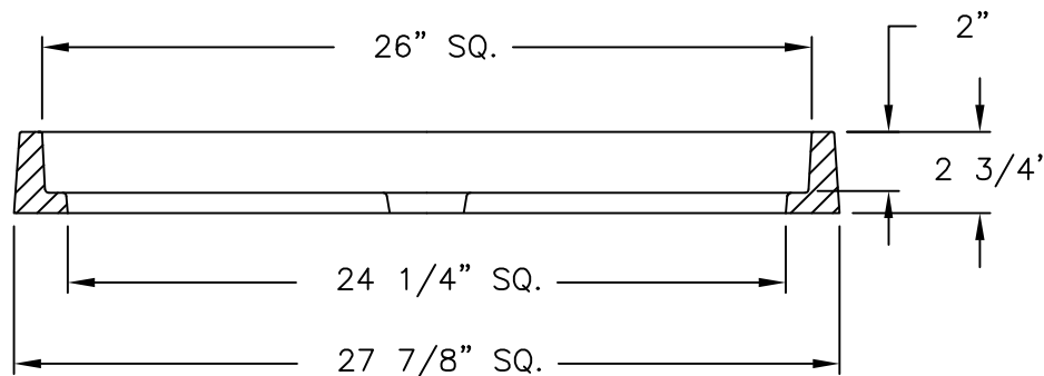
FRAME SECTION
