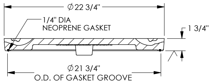
SECTION VIEW
