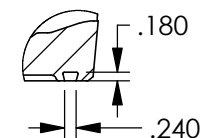
GROOVE DETAIL
