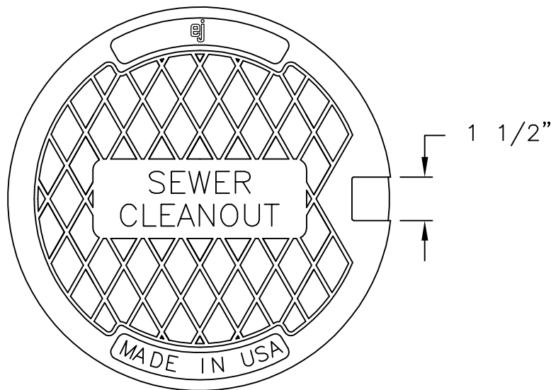
COVER FACE
