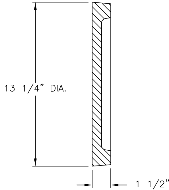
COVER SECTION
