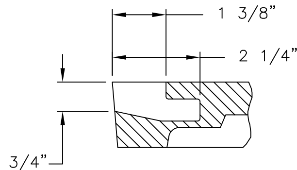
PICKHOLE DETAIL
