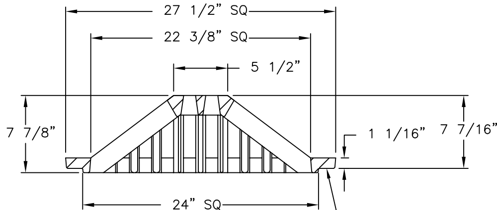
GRATE SECTION
