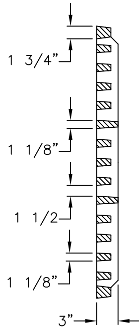
GRATE SECTION
