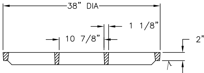
GRATE SECTION
