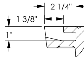
PICKHOLE DETAIL
