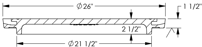
COVER SECTION
