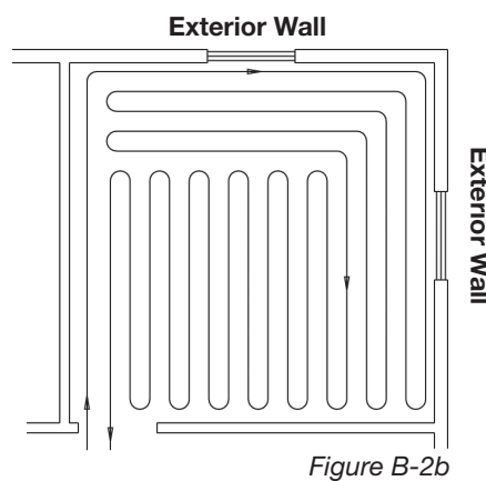
Figure B-2b Two-Wall Serpentine Room has two exterior walls
