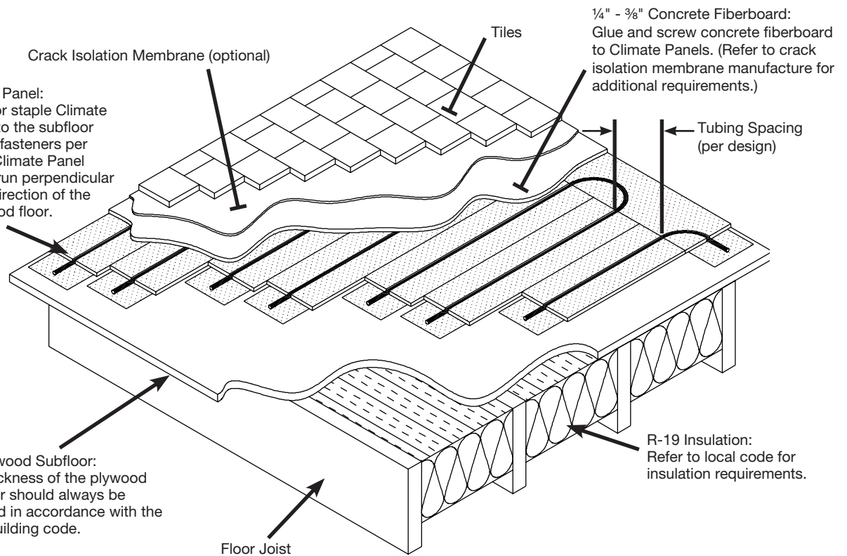
Figure A-2b Section through Climate Panel installation above subfloor with tiles
