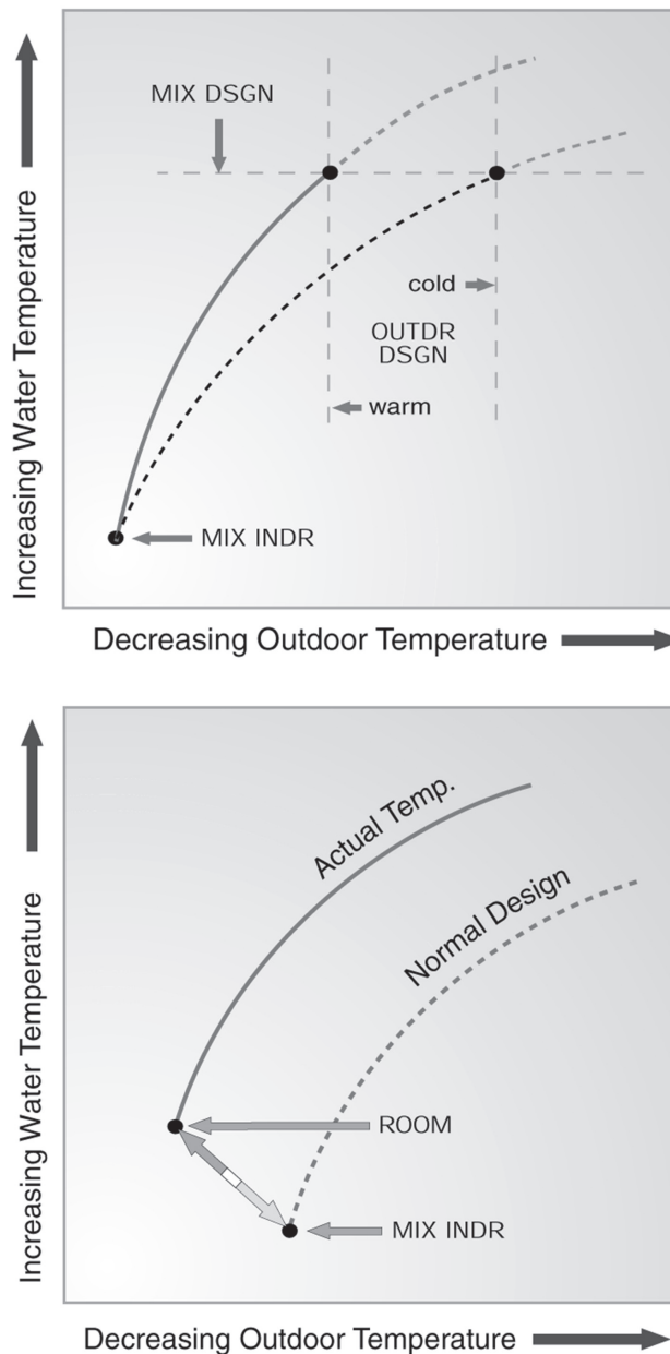
Figure 1-35 Outdoor reset curve
