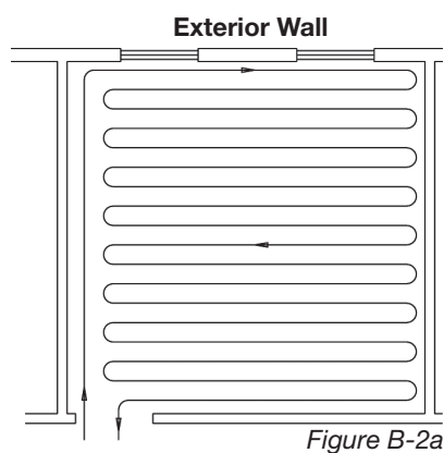
Figure B-2a One-Wall Serpentine Room has one exterior wall
