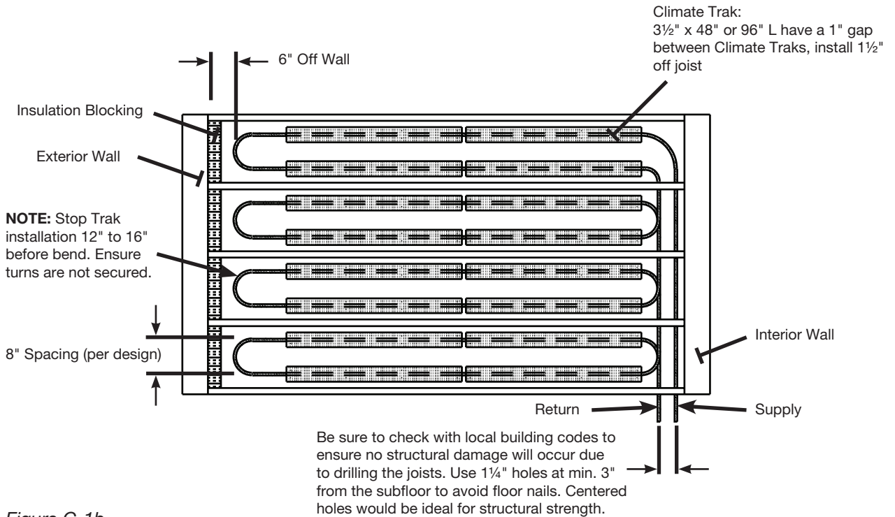
Figure C-1b Joist space layout -- Climate Trak
