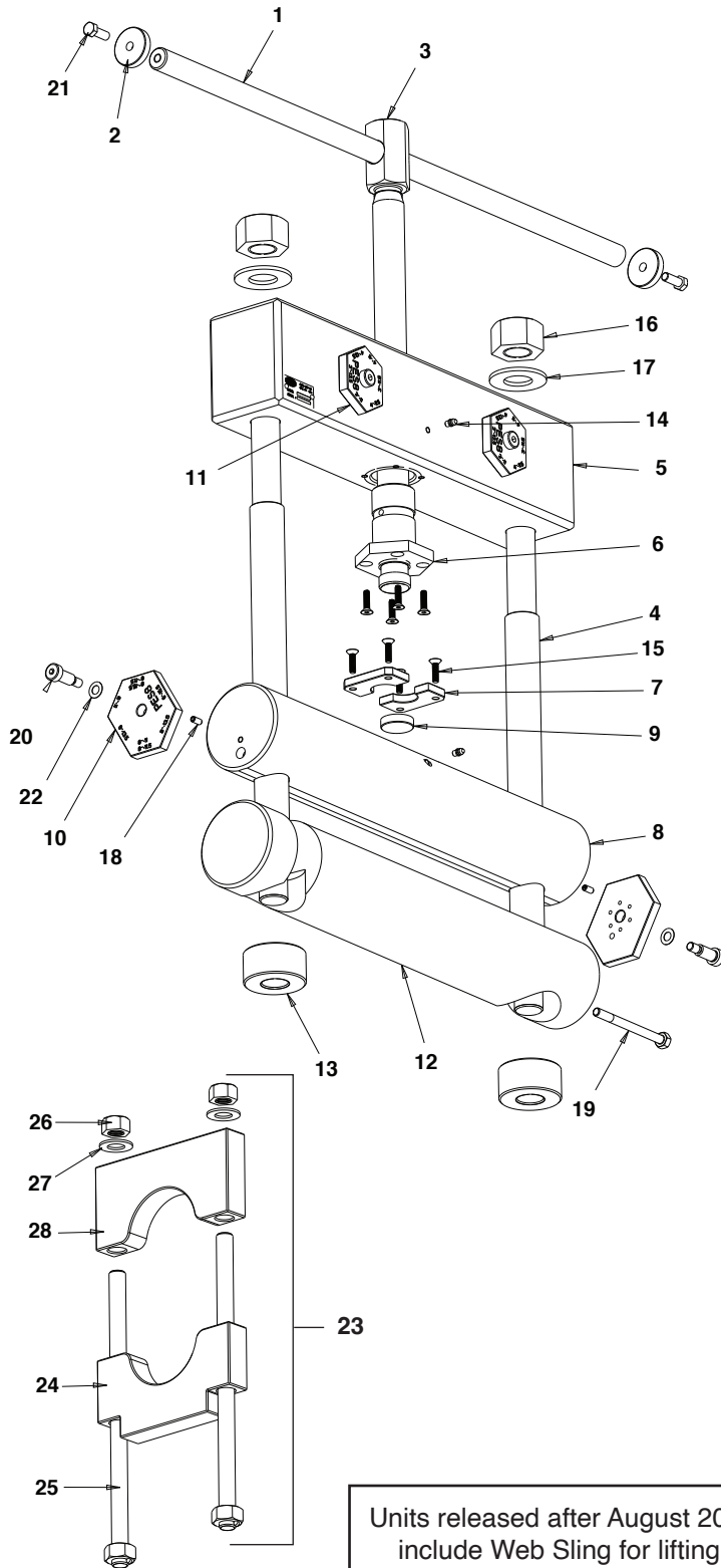
#04311 Clamp Assembly
