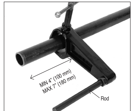
Fig. 5 Safety Arm Position. Rod on black safety arm helps resist the threading torque to protect the operator.
