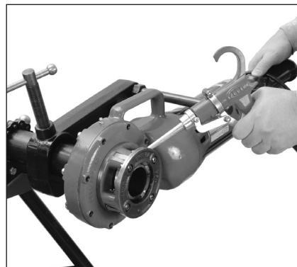
Fig. 4 Threading 2" Pipe.
