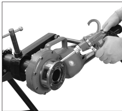
Fig. 4 Threading 2" Pipe.
