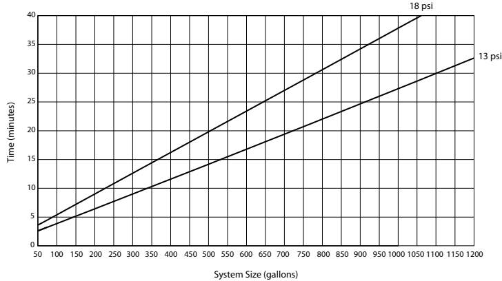
Estimated Time to Reach Various Pressures - Series 7C7 with 1/2-hp (110 VAC, 60-Hz) Compressor and Auto Vent
