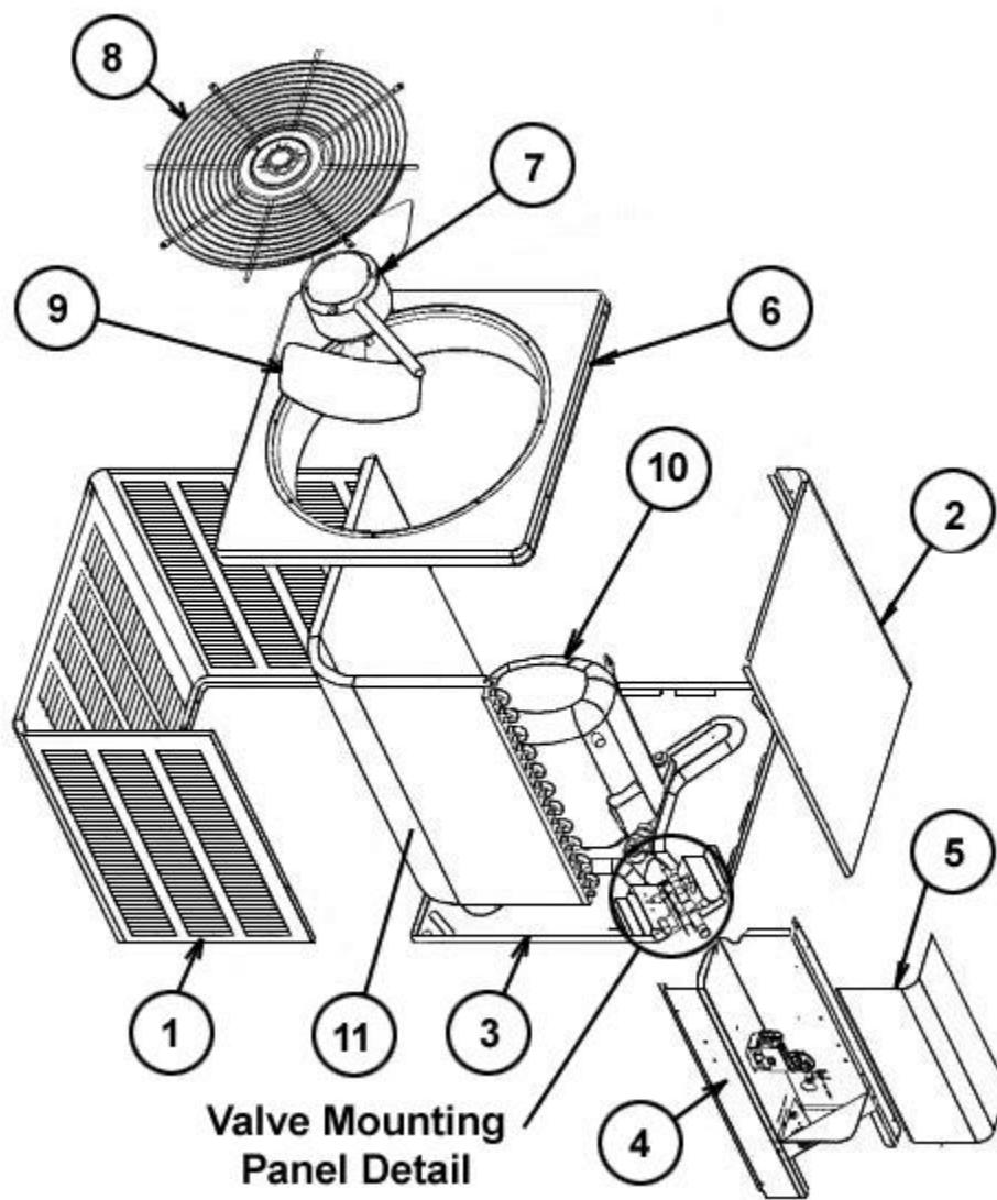
Exploded View
