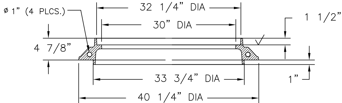
FRAME SECTION
