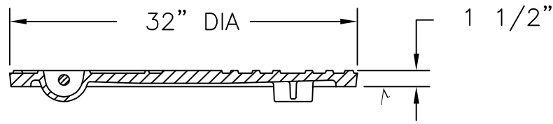
CROSS SECTION
