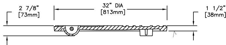
COVER SECTION
