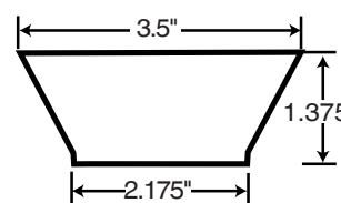
Standard 401 Style Skirt adjustable to 2" to 3" with standard cup (45-10-041)
