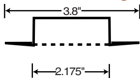
Flush Skirt adjustable 1/4" to 3/4" with short cup 1/4" to 1-5/8" with standard cup (45-10-051)
