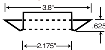
Short Taper Skirt adjustable 3/4" to 1" with short cup 3/4" to 1-7/8" with standard cup (45-10-061)
