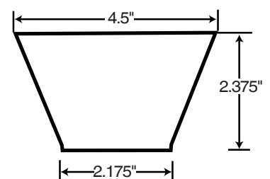
Extra Deep Skirt adjustable 3" to 5" with standard cup (45-10-047)
