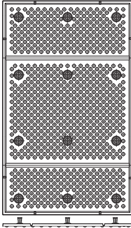
BOTTOM VIEW
