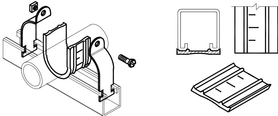
FIGURE 7862 - Pipe Wrap
