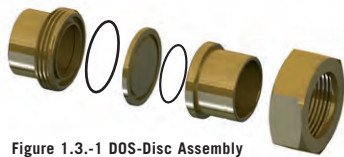
Figure 1.3.-1 DOS-Disc Assembly 1".....50013 3/4".....50014 1/2".....50016
