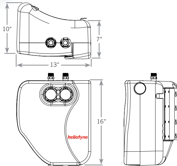
Figure 1B-1: HPAS Dimensions
