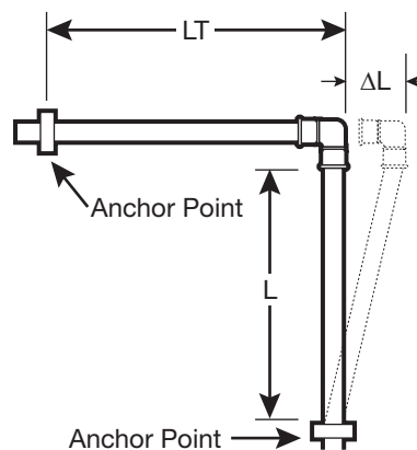
Corner Offset
