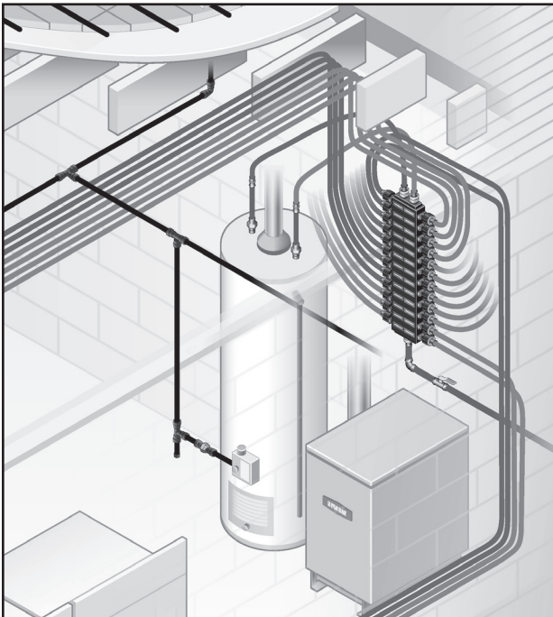
Figure 8.2 Combination Installation
