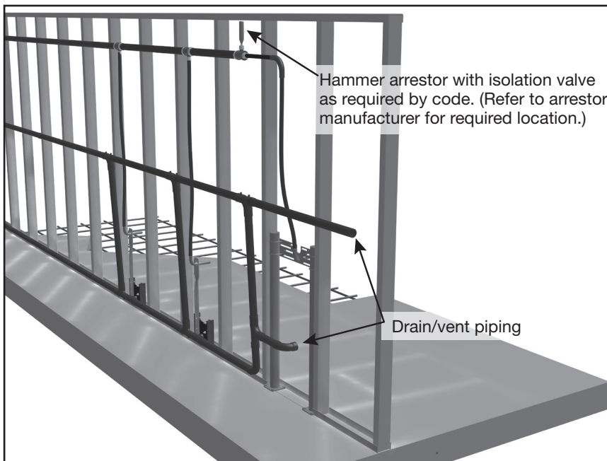
Figure 8.8 PureFlow PEX Piping to Flush Valves - Rear View
