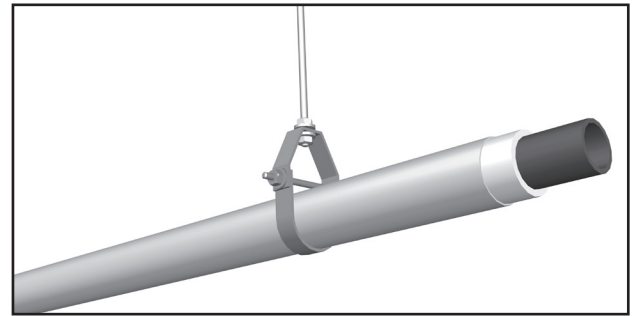
Figure 9.7 Typical PEX tubing support for clevis hanger
