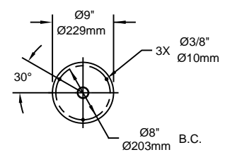
MOUNTING DETAIL B
