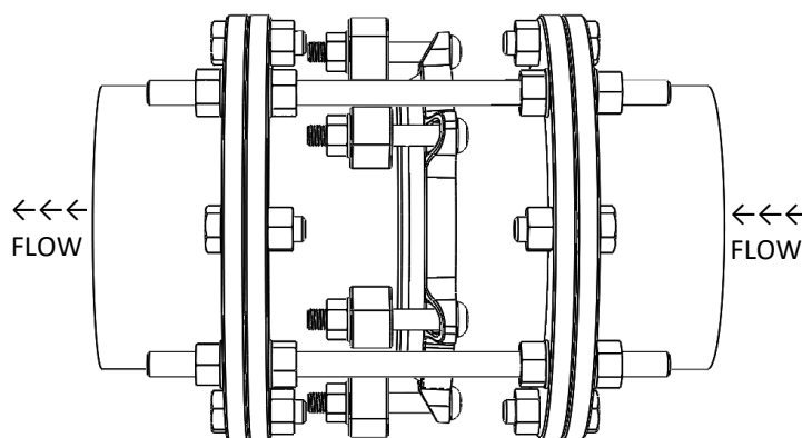
975 Restrained Dismantling Joint
