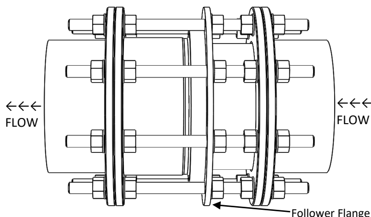
972 HD Restrained Dismantling Joint
