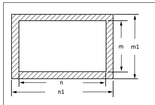
Cutout dimensions Starck K
