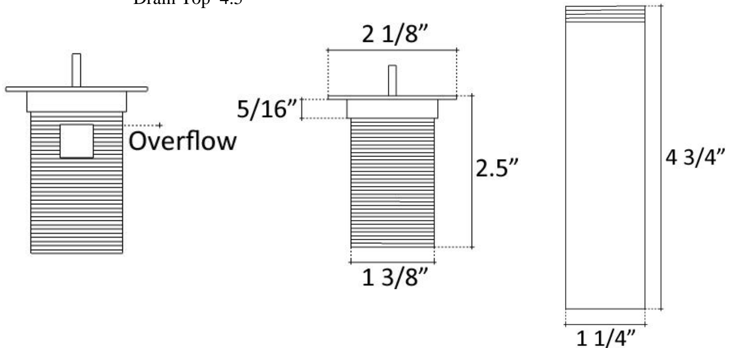
Drain Top 4.5"
