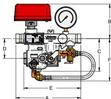
1 - 2"/25 - 50 mm Nominal Sizes
