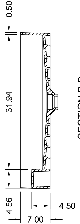
SECTION B-B
