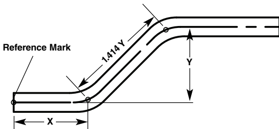
B – Bent Tube with Markings
