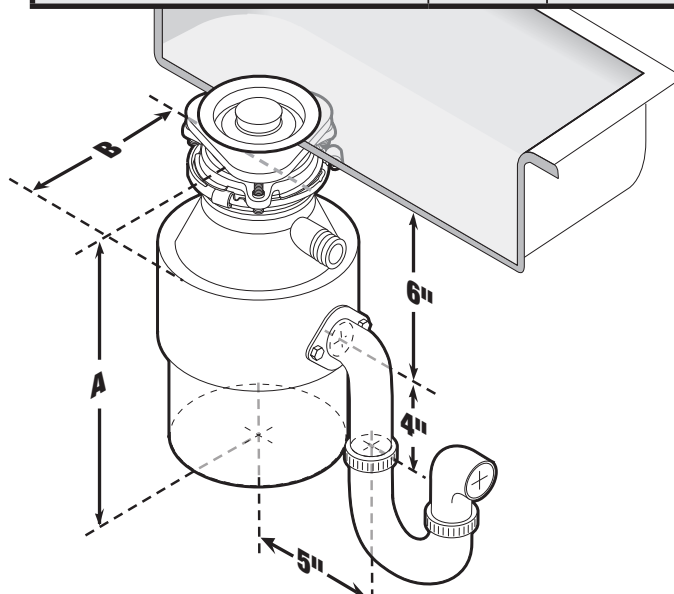
Dimensions/Dimensiones/Dimensions
