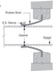
Manhole Detail A
