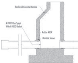
Manhole Detail B
