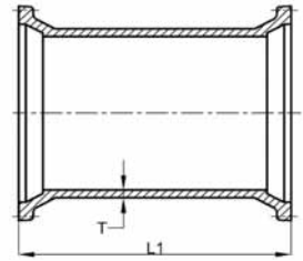
Short Sleeve
