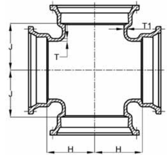
MJ Cross
