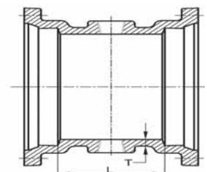
Tapped Cross
