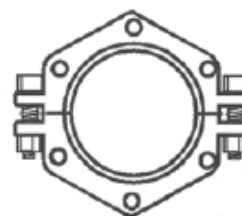
Swivel Gland
