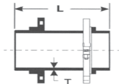
Swivel x Solid Adapter
