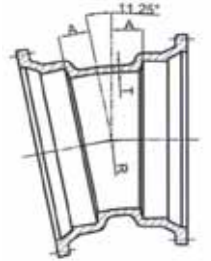
MJ x MJ 11-1/4° Bend
