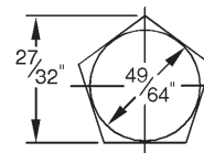
Standard waterworks
