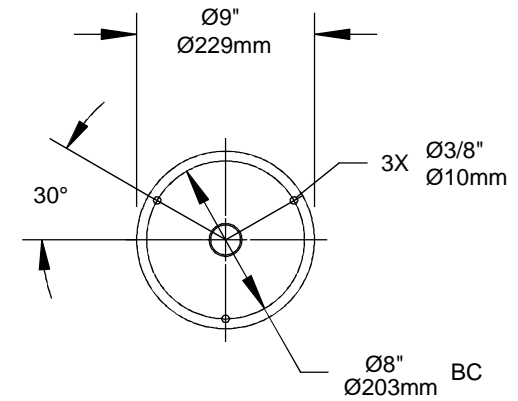
MOUNTING DETAIL
