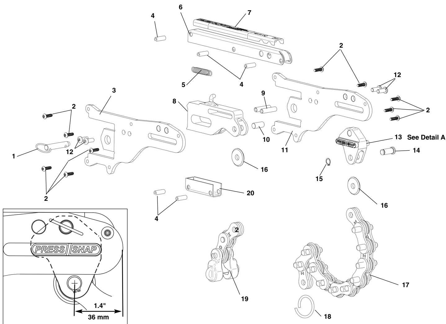
Detail A
