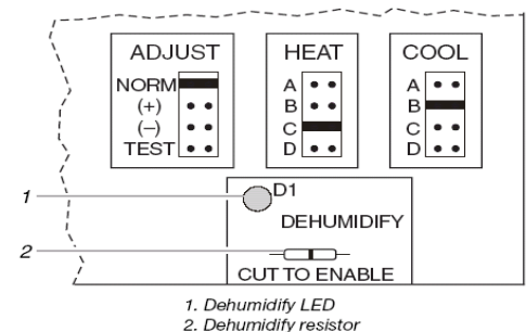
Control Board Taps and Dehumidify Resistor.
