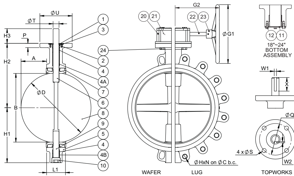
DIMENSIONS (INCHES) SIZES 14" – 24"
