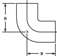
607-2-2 90° Fitting Elbow – Close Rough Ftg x Ftg – Wrot
