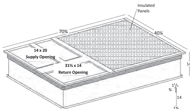
3-D VIEW
