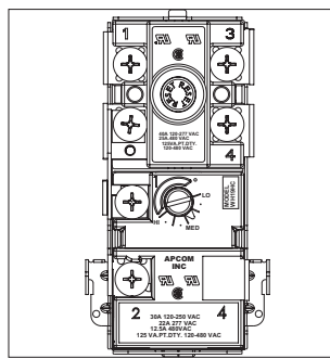
Figure 9. APCOM Thermostat Controls
