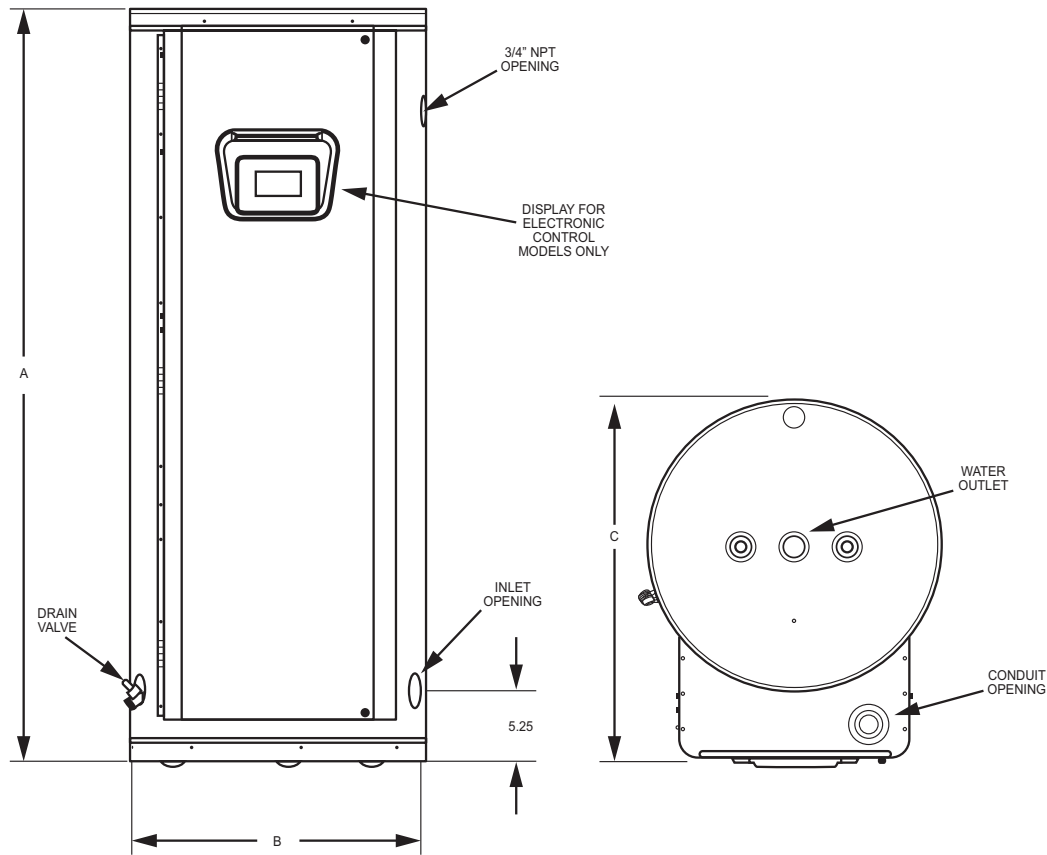
Figure 4. Rough-In Dimensions
