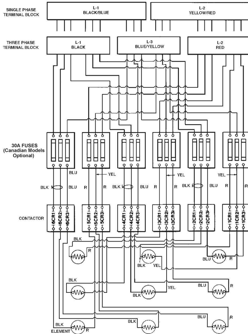
Figure 18. Nine-Element Single- and Three-Phase Power Circuits
