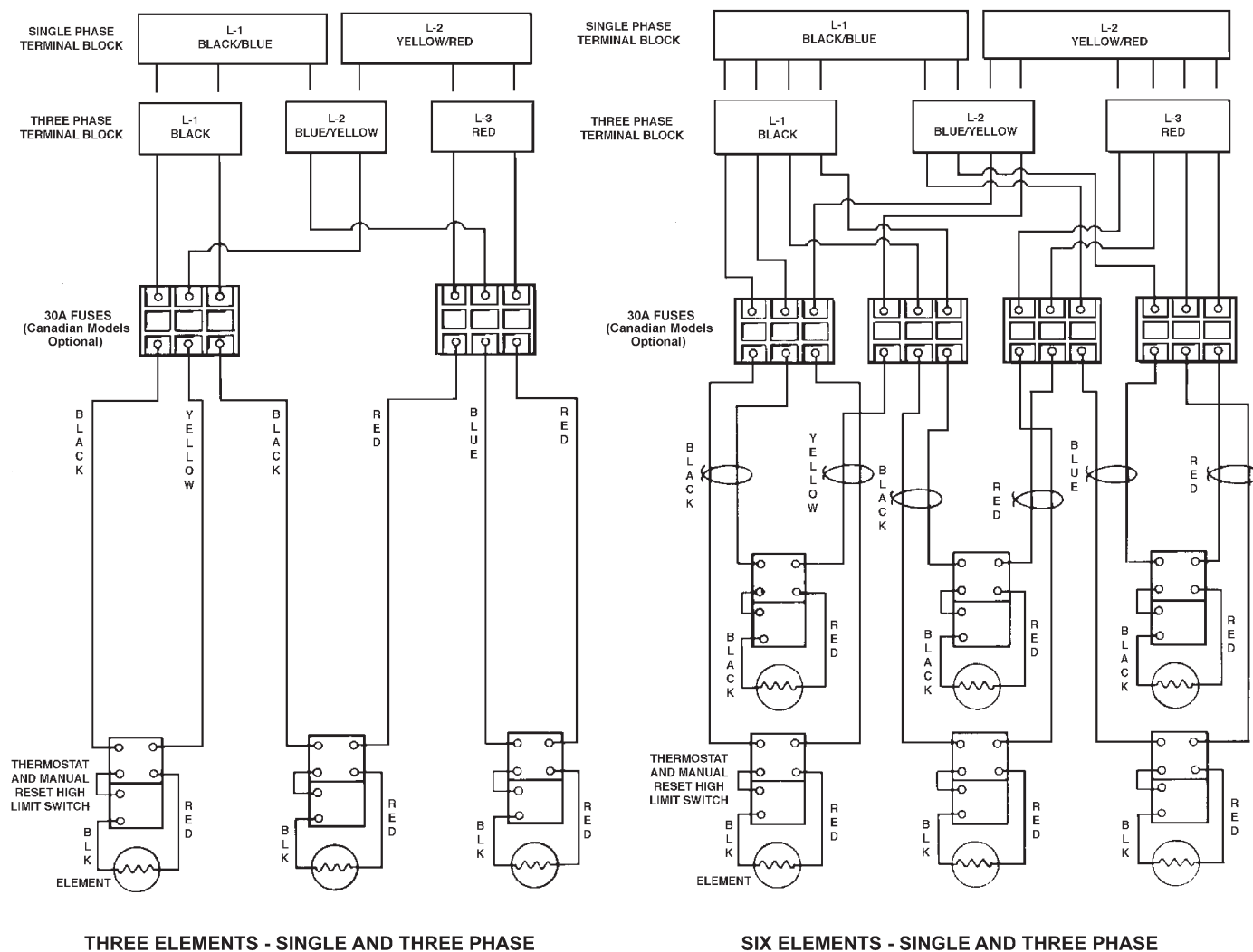
Figure 19. Three- and Six-Element Single- and Three-Phase Power Circuits
