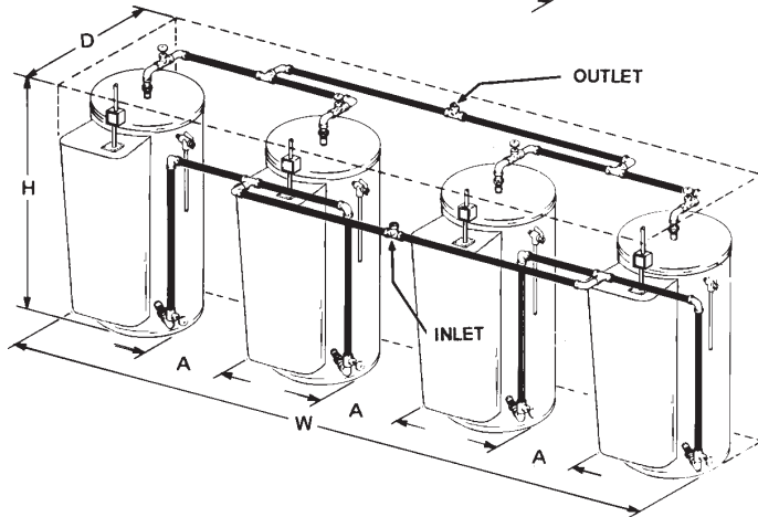
Figure 21. Manifold Kits
