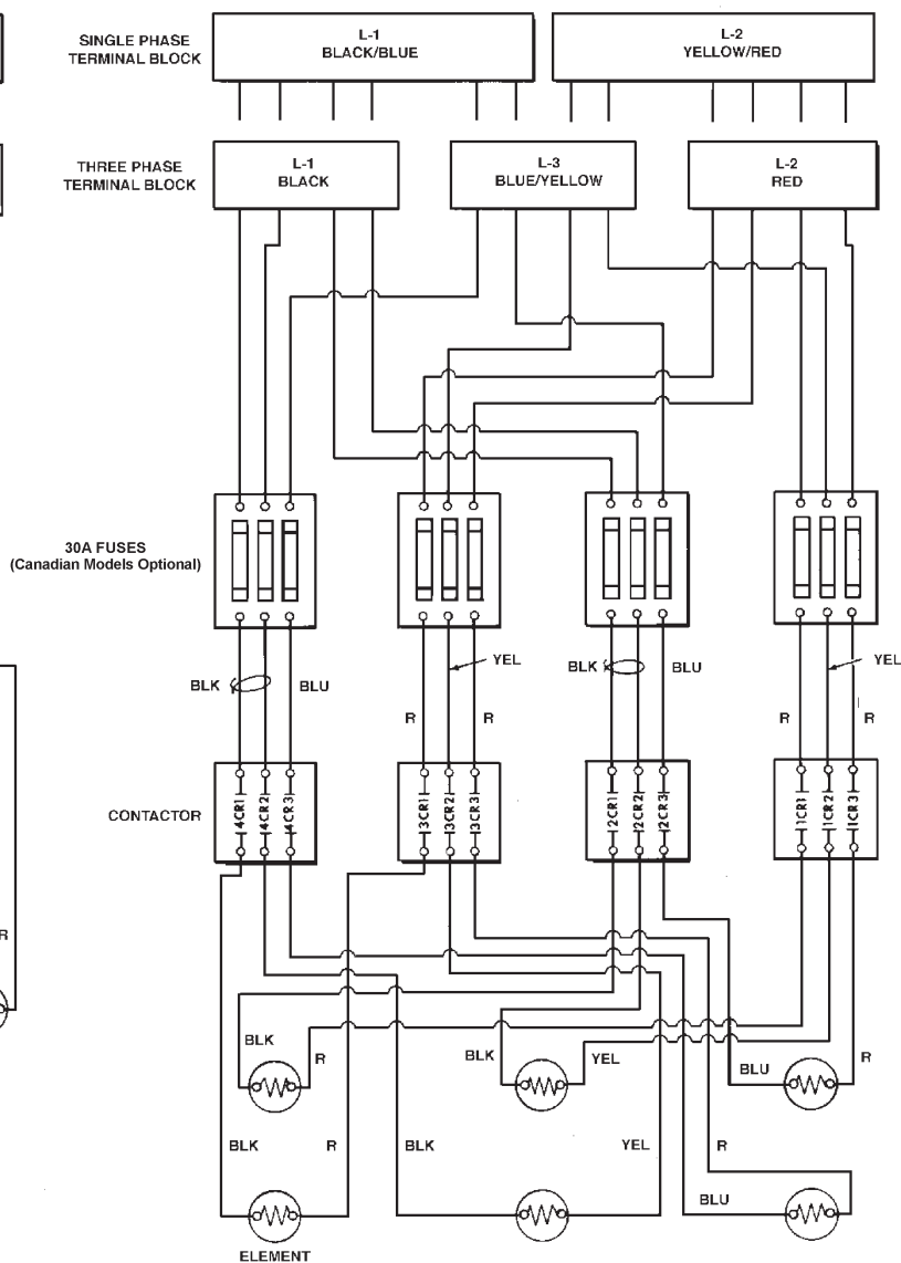
SIX ELEMENTS - SINGLE AND THREE PHASE
