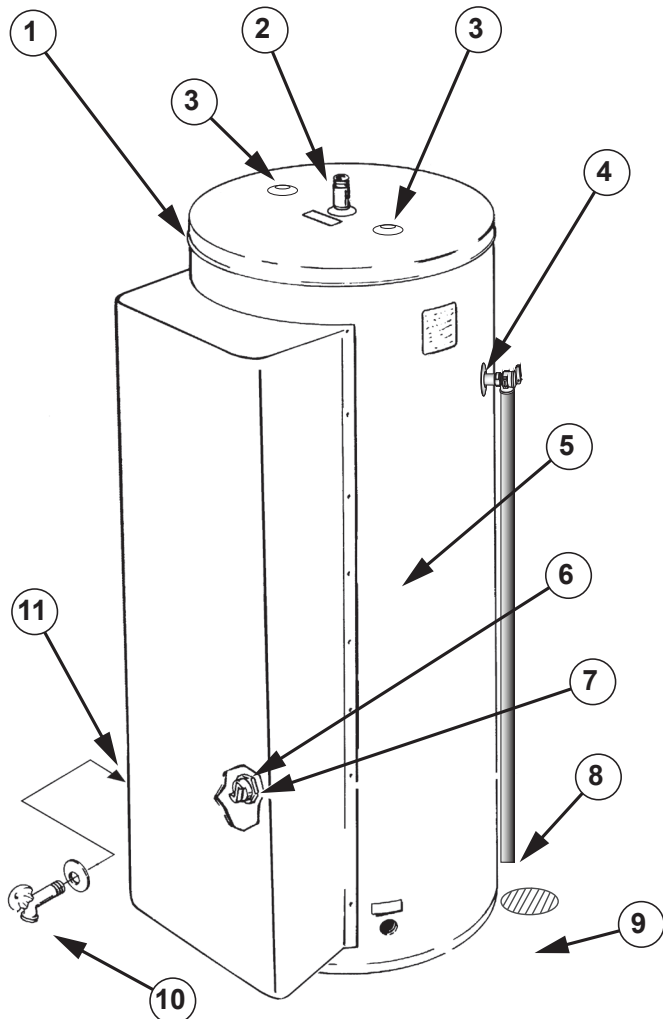
Figure 15. Leakage Checkpoints
