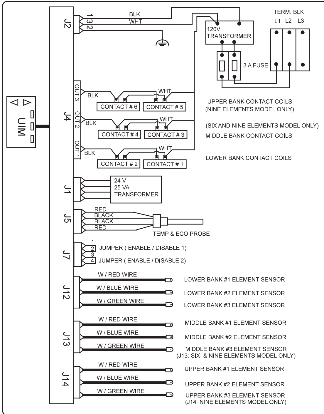
Figure 16. CCB (Central Control Board) Control Circuit Diagram - Electronic Control Models
