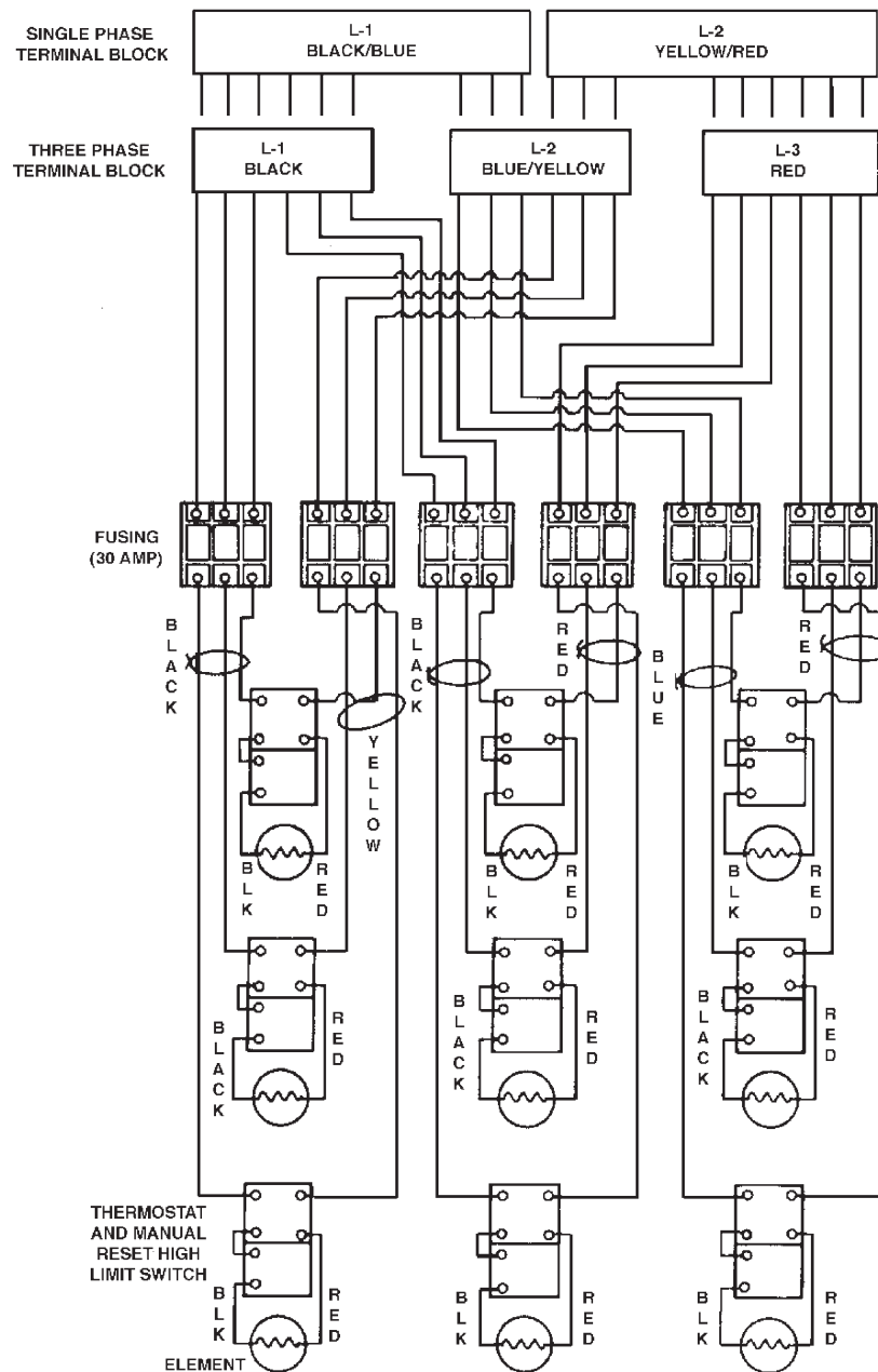
Figure 20. Nine Elements - Single And Three Phase
