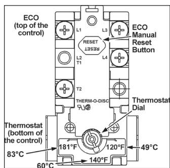
Figure 8. Thermodisc Thermostat Controls
