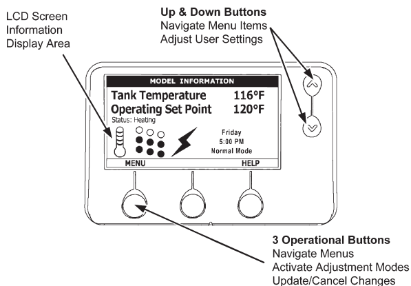
Figure 11. UIM - USER INTERFACE MODULE
