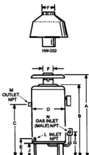
FIGURE 1. DIMENSIONS
