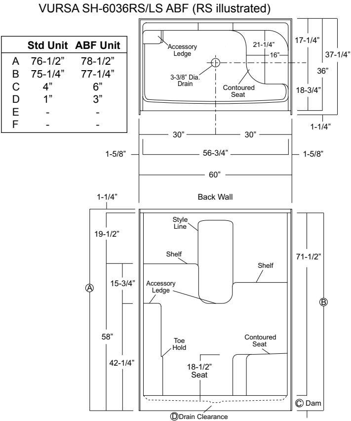
Illustration 1b - Center Drain, Unit Dimension & Alcove Framing Guidelines (dimensional tolerance +0 / -3/8")
