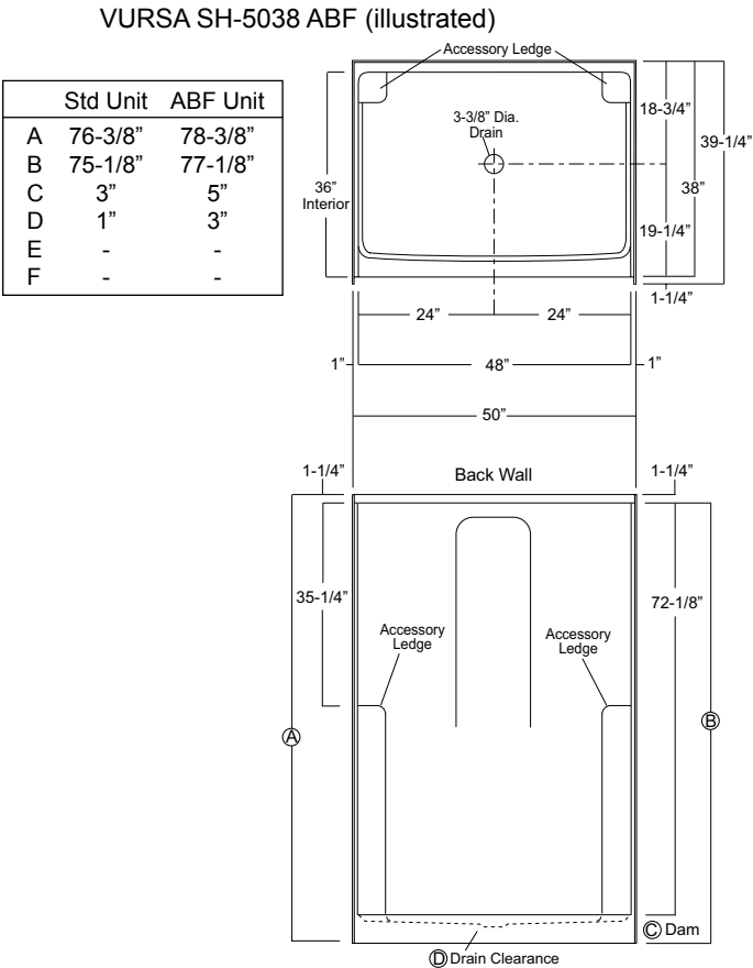
Illustration 1c - Center Drain, Unit Dimension & Alcove Framing Guidelines (dimensional tolerance +0 / -3/8")
