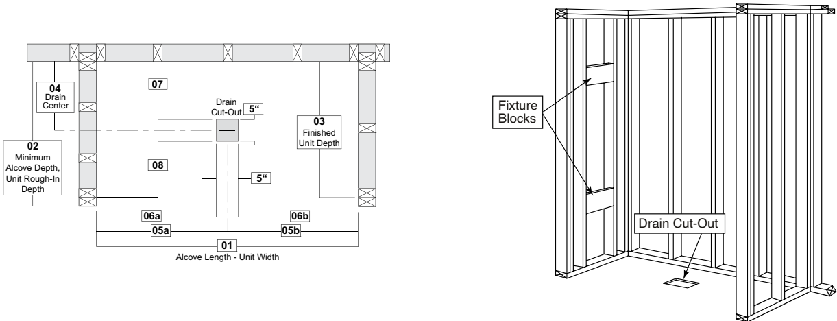
Illustration 1c - Center Drain, Unit Dimension & Alcove Framing Guidelines (dimensional tolerance +0 / -3/8")
