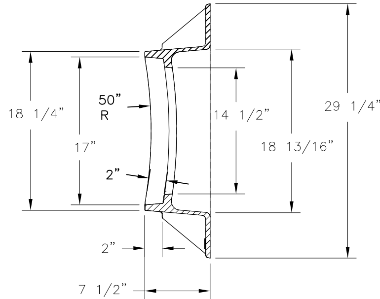
FRAME SECTION
