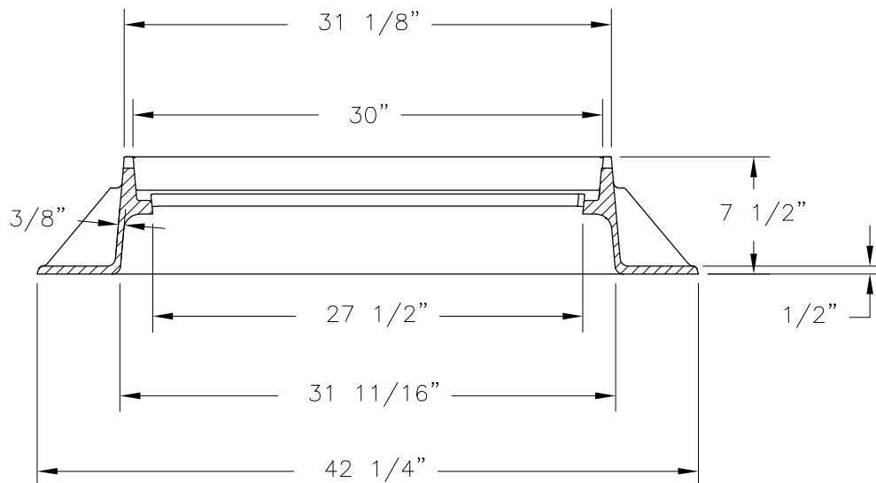
FRAME SECTION
