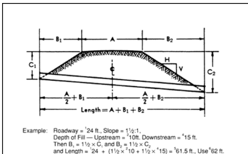
Figure 33. Computation of culvert length-flow line on steep grade.
