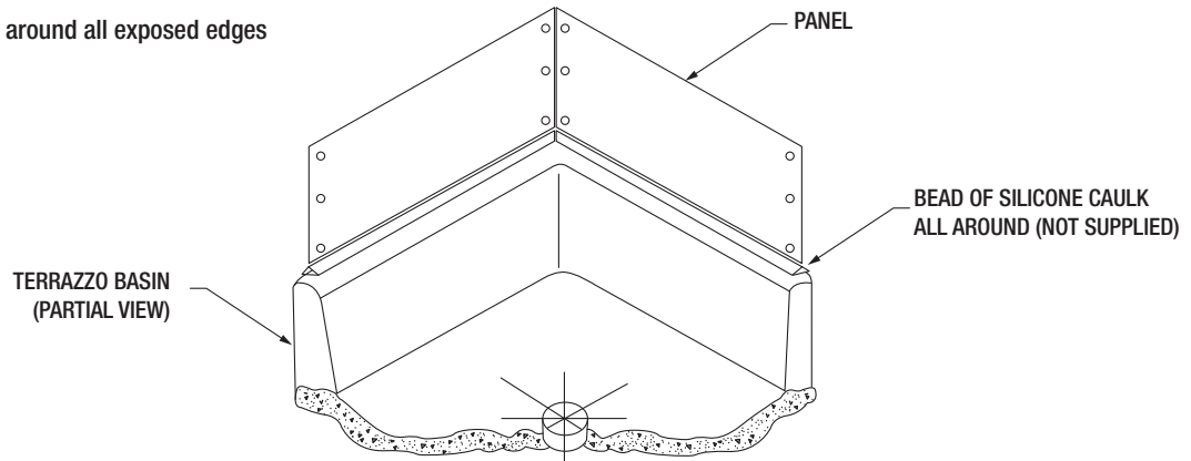
2 PANELS REQUIRED
