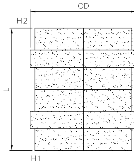
FABRICATED FITTING (F1)
