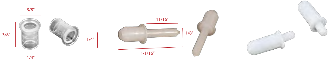
Flange Bushing
