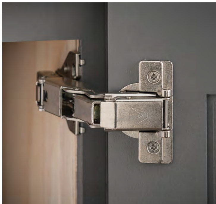
Full Overlay 0 mm Crank
