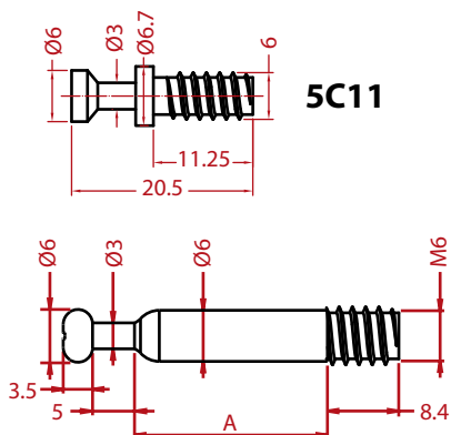
Connecting Bolt
