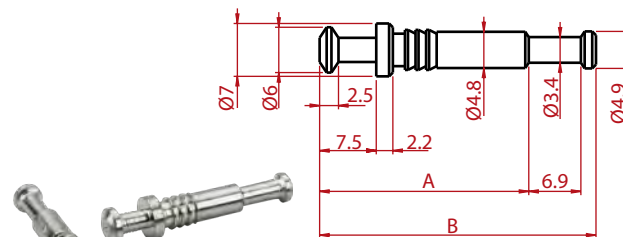
Center Panel Double Bolt
