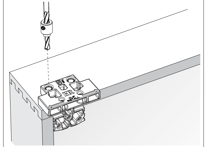
Drilling Location for Rear Hook Hole on Drawer Box; Left and Right
