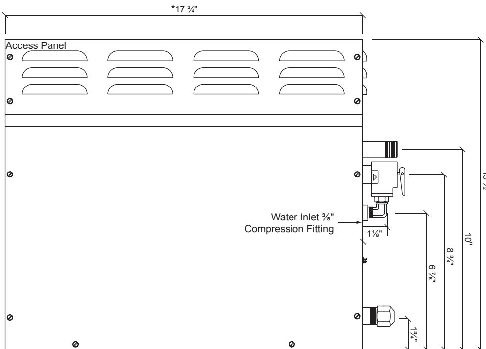
Front Access
