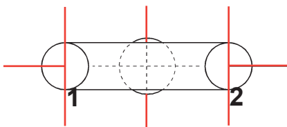
Right angle "U" branch - top right illustration: viewed from inlet end; bottom right illustration: viewed from outlet end
