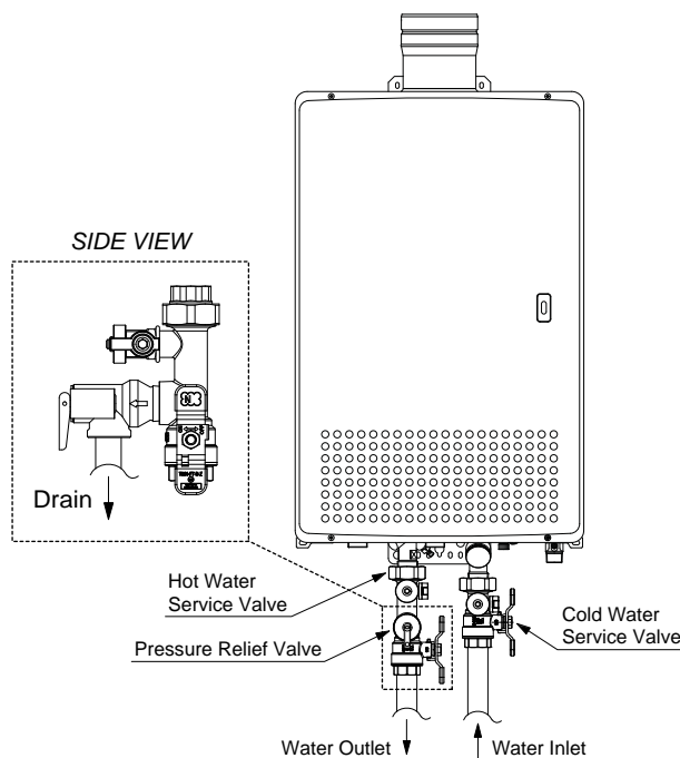
Figure 2. Completed Installation
