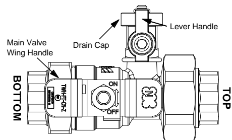
Figure 1. Valve Detail (Cold Water Valve shown)
