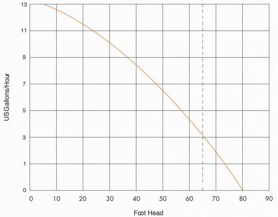
Plot of FlowRate Against Head
