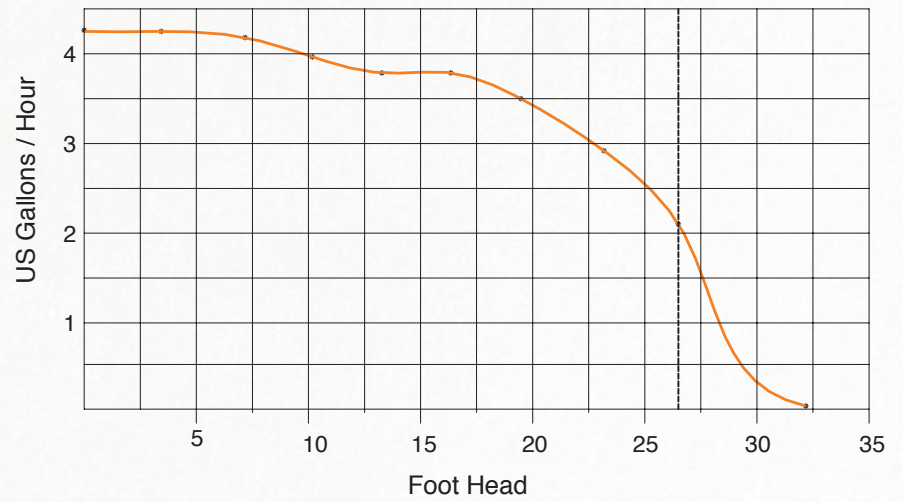
Plot of Flow Rate Against Head
